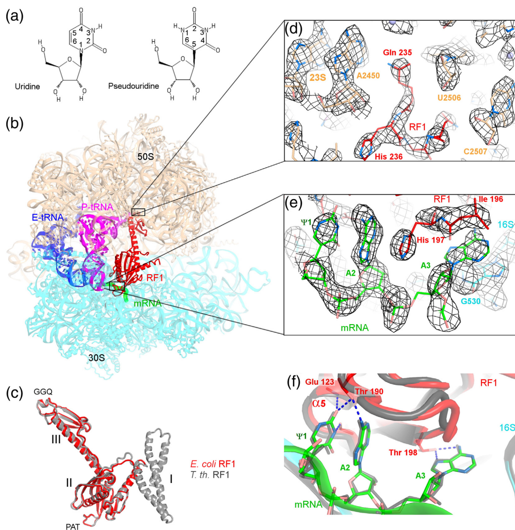
Fig. 1. Structural basis for recognition of the ΨAA codon by RF1. (a) Chemical structures of pseudouridine and uridine. (b) Crystal structure of the 70S•ΨAA•RF1 termination complex (this work). The 50S subunit is shown in wheat and 30S subunit in cyan. (c) Similar conformations of E. coli (this work) and T. thermophilus release factors in 70S termination complexes. (d–e) Unbiased feature-enhanced density map [37] shows well-resolved features of RF1 in the peptidyl-transferase center in (d) and ΨAA and RF1 in the decoding center in (e). (mRNA and RF1 were not included in the simulated-annealing-refined 70S model used for map calculation.) (f) Comparison of the conformations of the ΨAA (this work) and UAA (gray) codons in the 70S•RF1 termination complexes. In panels (c) and (f), the structure of T. thermophilus 70S•RF1 complex (PDB ID: 4V63, [11]) is shown in gray.
