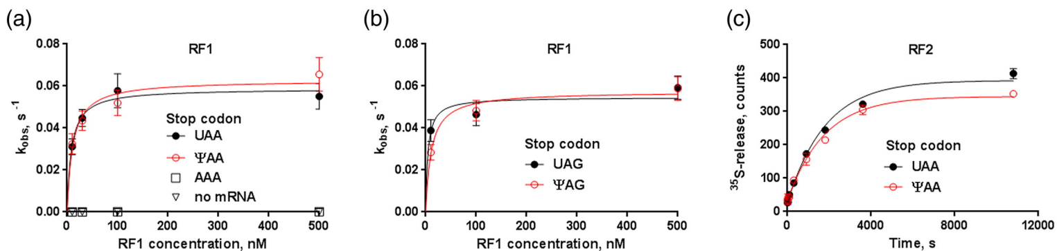
Fig. 3. Kinetics of peptide release from 70S ribosomes programmed with pseudouridylated stop codons are similar to those with non-modified stop codons. (a) Michaelis–Menten curves for RF1-mediated release of [^{35}\text{S}] -fMet from E. coli ribosomes programmed with the stop codons UAA (filled circles) or \Psi AA (clear circles, red curve), sense codon AAA (clear squares), or not bound with an mRNA (clear triangles). (b) Michaelis–Menten curves for RF1-mediated release of [^{35}\text{S}] -fMet from E. coli ribosomes programmed with the UAG (filled circles) or \Psi AG (clear circles, red curve) codon. (c) Time progress curves for RF2-mediated release of [^{35}\text{S}] -fMet from E. coli ribosomes programmed with the UAA (filled circles) or \Psi AA (clear circles, red curve) codon at 10 nM RF2.
