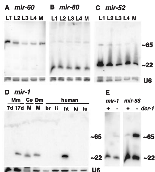
Fig. 1. Northern blots of small RNA transcripts. (A through C) Total RNA from C. elegans larvae (stages L1 through L4) or from mixed stage (M) populations were blotted and probed with oligonucleotides complementary to either the 5' or 3' half of the indicated transcript (13). U6 = the same filters were probed with probe to U6 snRNA as a loading control. (A) mir-60 5' probe detects a transcript of ~65 nt. The ratio of L1 to L4 mir-60 signal, normalized to U6, is about 5:1. The mir-60 3' probe (not shown) detects a similar-sized species with a similar developmental profile. (B) mir-80 3' probe detects a ~22-nt RNA expressed uniformly at all stages. (C) mir-52 5' probe. The normalized mir-52 signal is three-fold greater in the L1 versus the L3. (D) mir-1 3' probe detects a transcript of ~22 nt in total RNA from mouse (Mm) 17-day embryos, mixed-stage C. elegans (Ce), Drosophila melanogaster (Dm) mixture of embryo-larvae-pupae, and in a sample of human heart (ht) tissue. Other human tissue samples were brain (br), liver (li), kidney (ki), and lung (lu). (E) mir-1 and mir-58 probes to total RNA from mixed populations of wild-type (+) and dcr-1(ok247) (-) animals. An increase in the proportion of unprocessed ~65-nt precursor is observed in the dcr-1 RNA.
