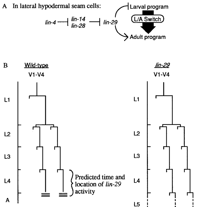
Fig. 1. Temporal control of the lateral hypodermal cell terminal differentiation. (A) Epistasis relationships among four heterochronic genes (Ambros, 1989). Briefly, lin-29 activity is required at the final molt of the worm for the repression of larval-specific developmental programs and activation of adult-specific programs in lateral hypodermal cells. Genetically, lin-14 and lin-28 act as negative regulators of lin-29 activity. Down-regulation of these two genes by the action of lin-4 on lin-14 is required for proper temporal activation of lin-29 . (B) The cell lineage of lateral hypodermal seam cells V1-V4 in wild-type and lin-29 mutant worms (Sulston and Horvitz, 1977; Ambros and Horvitz, 1984). The vertical axis represents time, with a hatch-mark to indicate each molt. L1-L4 indicate the 4 wild-type larval stages; A indicates the adult stage. L5 represents supernumerary larval stages that occur in the absence of lin-29 activity. In the lineage diagram, the horizontal lines indicate cell divisions. In wild-type animals, seam cells divide during the first three molts and then terminally differentiate during the fourth molt, as indicated by the triple horizontal lines. In lin-29 mutants, seam cell divisions continue during the fourth and subsequent (L5 etc.) molts, and the cells remain larval in character. Wild-type lin-29 activity is predicted to be required during the L4 stage to trigger the L/A switch.
