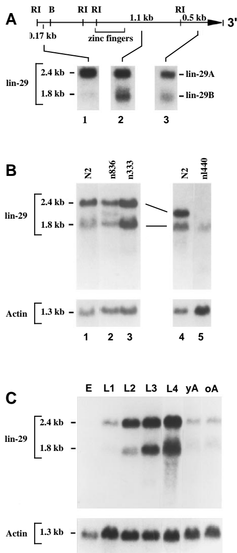
Fig. 3. Northern analysis of lin-29 transcripts. Poly(A) + RNA was isolated from developmentally staged worm populations and analyzed by northern hybridization. Transcript sizes were estimated based on ethidium bromide staining of the 18S and 28S ribosomal RNAs in a sample of total RNA run on the same gel. (A) A restriction map of lin-29A cDNA is shown indicating the different fragments used to probe a northern blot. RI, EcoRI ; B, BstEII . Below the map are autoradiographs of a northern blot of L4-stage RNA hybridized sequentially with three different fragments: the 5' 0.17 kb EcoRI - BstEII fragment (Lane 1), the 1.1 kb EcoRI zinc finger containing fragment (Lane 2), and the 3' 0.5 kb EcoRI fragment (Lane 3). (B) RNA isolated from synchronized L4-stage populations of wild-type N2 (lanes 1 and 4), and three lin-29 mutants, n836 (lane 2), n333 (lane 3) and n1440 (lane 5), was analyzed by northern blot. Lanes 1-3 and lanes 4 and 5 are from two separate experiments. In each case, the upper autoradiogram is an exposure of a filter hybridized with the 1.1 kb EcoRI fragment of lin-29 , and the lower autoradiogram is the same filter rehybridized with an act-1 probe (Files et al., 1983) as a control for amounts of RNA loaded. (C) RNA was isolated from staged populations as indicated and analyzed by northern hybridization using the 1.1 kb EcoRI fragment as probe. E, RNA isolated from mixed-stage eggs; L1-L4, the four larval stages; yA, young adults containing no or just a few eggs; oA, older gravid adults. The lower autoradiogram is the same filter hybridized with an act-1 probe (Files et al., 1983).
