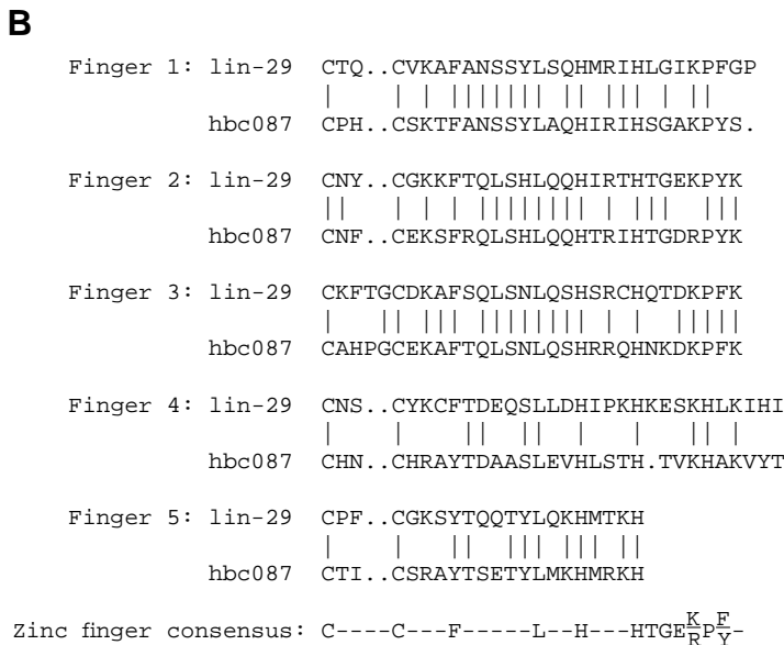
Fig. 5. Comparison of the five lin-29 zinc fingers with the (Cys) 2 -(His) 2 zinc finger consensus. (A) The consensus sequences for the (Cys) 2 -(His) 2 zinc finger DNA binding motif and for the 'H/C link' sequence that joins adjacent zinc fingers (Berg, 1993; Schuh et al., 1986) are aligned with the five lin-29 zinc finger domains (numbered as in Figs 2, 4). Identical residues are highlighted in bold. Residues that occur in at least three of the five lin-29 fingers are outlined. (B) The amino acid sequence of the Lin-29 zinc finger motifs are aligned with those of the zinc fingers encoded by the human cDNA clone hbc087 (Takeda et al., 1993). Identical amino acids are indicated by vertical lines. In each figure, the dashes in the consensus represent any amino acid and the periods indicate gaps in the sequence.
