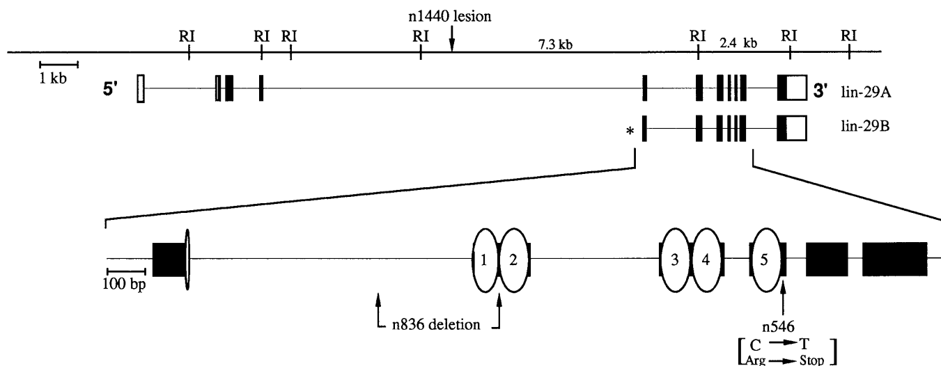
Fig. 2. lin-29 genomic region. The top line shows the lin-29 locus relative to EcoRI sites (RI). The two lin-29 primary transcripts, lin-29A and lin-29B are indicated below the line. Transcription is shown left to right for ease of comparison with Figs 4 and 5. This is in opposite orientation relative to the genetic map (Papp et al., 1991). Exons are indicated by boxes. Open boxes indicate 5' and 3' untranslated regions and the shaded boxes indicate coding regions. The * indicates that two 5'-ends of the lin-29B transcription unit have been identified by cDNA analysis (see text). In one, SL1 is trans -spliced to the start of Exon V of lin-29A . In the second, a 37 bp exon is cis -spliced to Exon V. The numbered ovals in the region expanded at the bottom of the figure indicate the positions of the five zinc fingers, with the numbers corresponding to those in Figs 4 and 5. The first six amino acids of zinc finger 1 are separated from the rest by an intron. The positions of the molecular lesions of three lin-29 mutations, lin-29(n546) , lin-29(n836) and lin-29(n1440) , are indicated.
